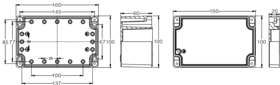
CRADYBOX-AL-160X100X80 - 0186004
